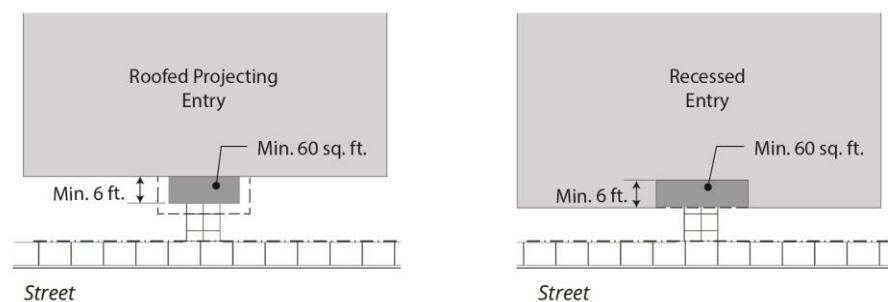
FIGURE 17.56.030.F-1: ENTRY PROTECTION
