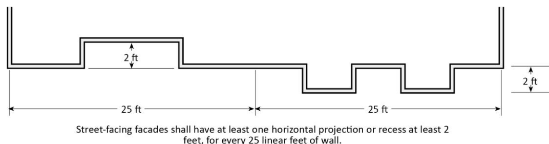
FIGURE 17.56.030.D-1: WALL FACADES
